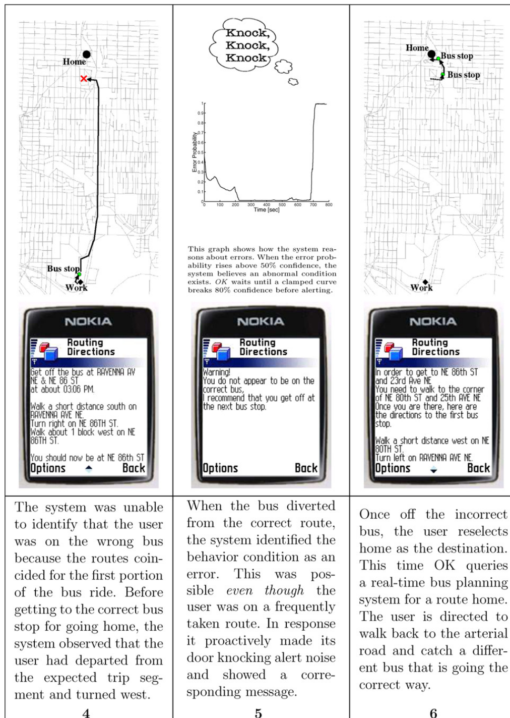
Fig. 9. An experiment using Opportunity Knocks (Part II).
