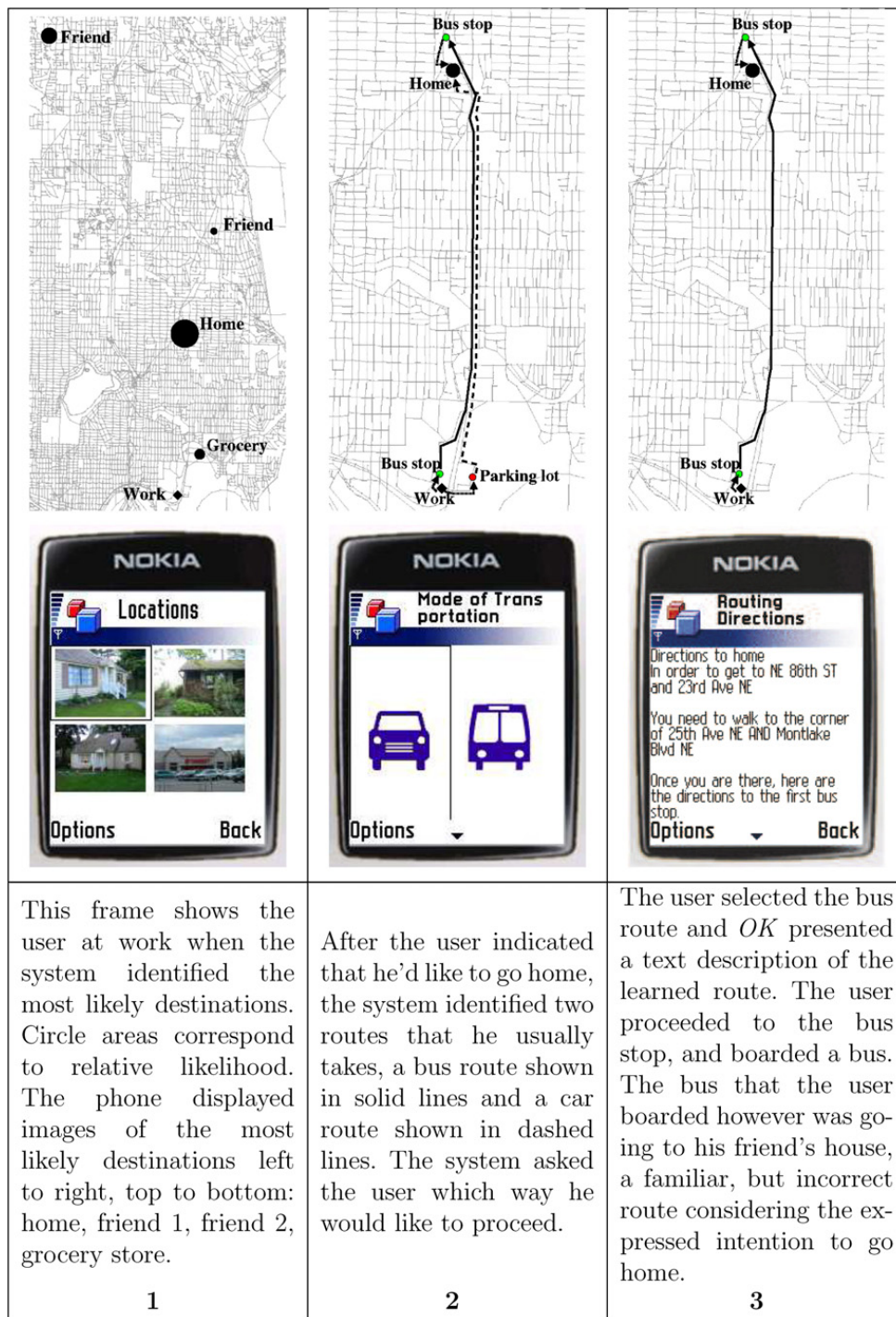
Fig. 8. An experiment using Opportunity Knocks (Part I).
