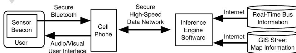
Fig. 7. The client-server architecture of Opportunity Knocks.
